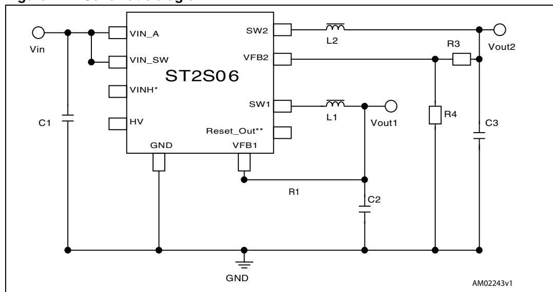
Figure 1. Schematic diagram
